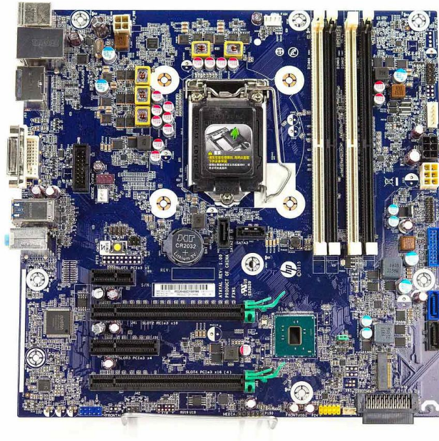
HP Z240 Workstation Motherboard (Refurb)
