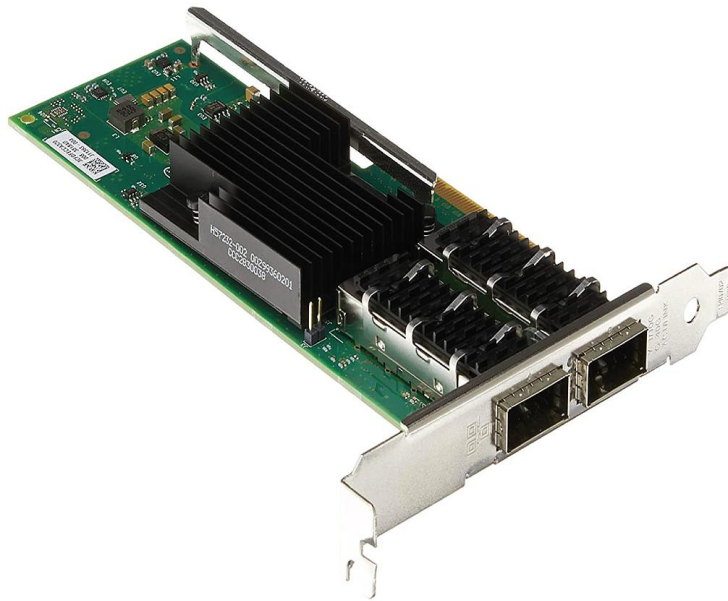
Intel XL710 10GbE SFP+ x 2 Ethernet Converged Network Adapter
